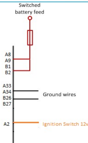
Figure 0-1 - Power Feeds and a Common grounding point.
