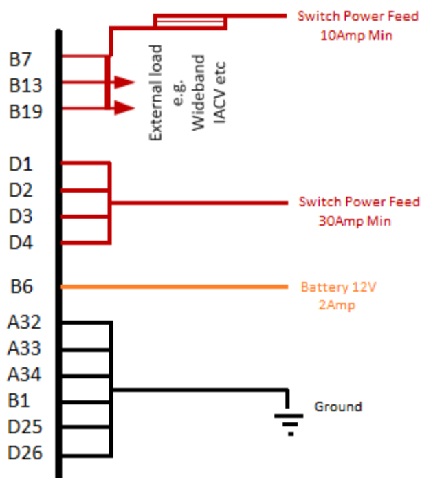
Figure 0-1 - Redundant Power Feeds and a Common grounding point.
